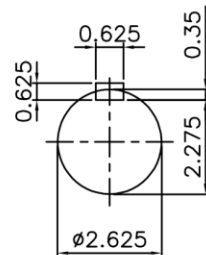
VIEW "A"
