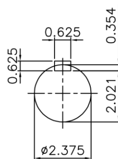
VIEW "A"
