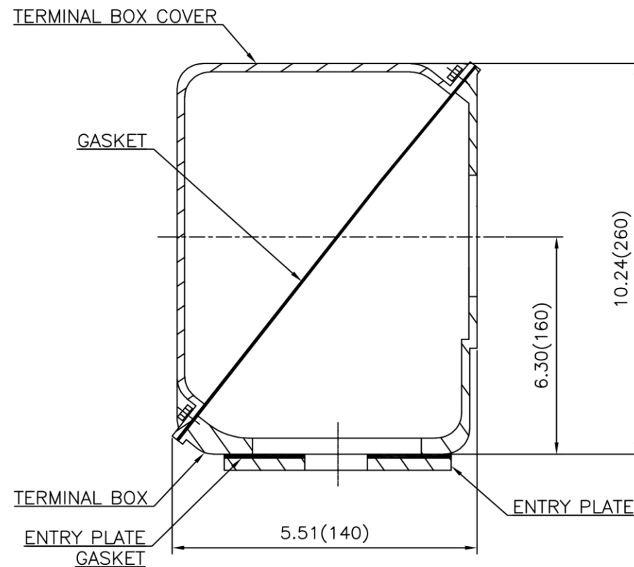
SEC. "A"—"A"
