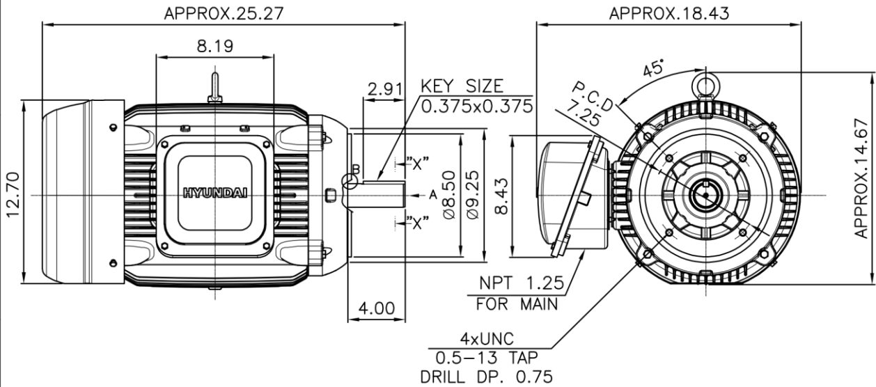
VIEW "A"
